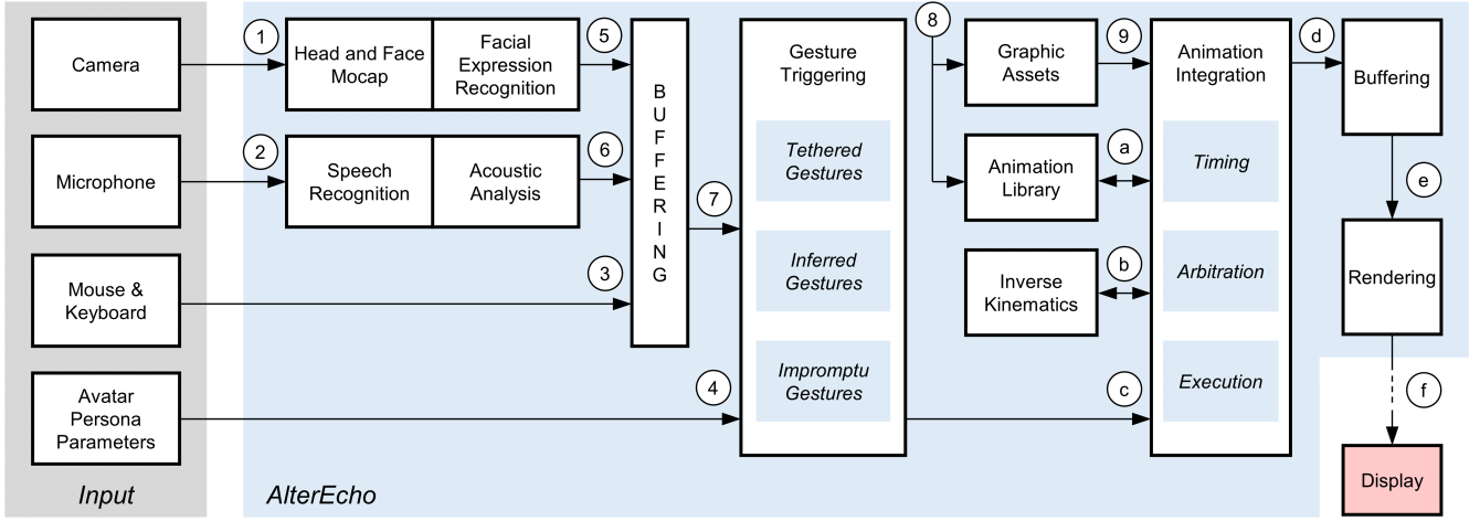
Figure 2: AlterEcho architecture.
