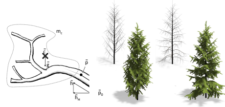
Figure 16: Heavy branches can bend down because of the weight.
