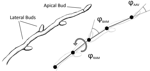
Figure 4: Various parameters affect shoot growth: bending angle \varphi_{BAM} , roll angle \varphi_{RAM} , and apical angle variance \varphi_{AAV} .
