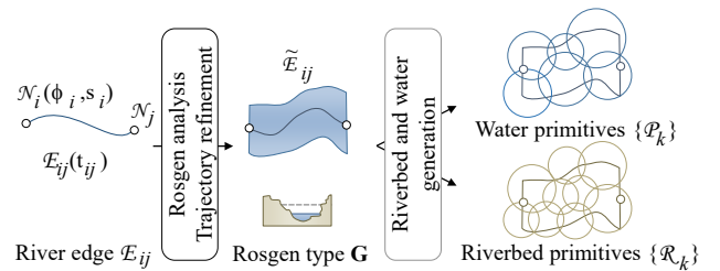
Figure 6: Our procedural amplification takes a coarse river trajectory \mathcal{E} and refines it according to the Rosgen type. Riverbed primitives \mathcal{R} for geometry carving and riverflow primitives \mathcal{P} for water animation are then seeded over the river domain.
