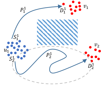
Figure 4: Source and Destination Clustering. Spatial clustering determines clusters u_1 , v_1 , and v_2 which are then used to form the two CMMs \{S_1^1 = u_1', P_1^1, D_1^1 = v_1\} and \{S_2^1 = u_1'', P_2^1, D_2^1 = v_2\} where u_1' is the subset of u_1 that navigates to v_1 and u_1'' = u_1 - u_1' .
