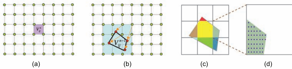
Figure 6: Control volume advection and mass transport in 2D. (a) The spatial domain is discretized into control volumes sharing corner points. (b) Control volume V_i^n advected back in time. Intersecting cells are shaded in light blue. (c) Intersection regions of V_i^{n-1} . (d) The local density distribution function is integrated over the intersection region using Riemann sum on sample points (purple).
