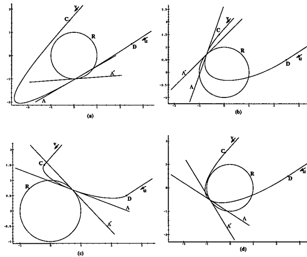
Figure 8: (a),(b): Two solutions for a conic arc that blends two segments and forms a 45^\circ angle with a line. (c),(d): Two solutions for a conic arc that blends two parallel segments and forms a 45^\circ angle with a line.
