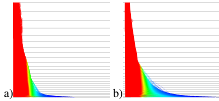
Figure 1: a) A histogram for the entire U.S. in early May. b) A histogram for late August. Notice how the CO 2 values have shifted to the right.
