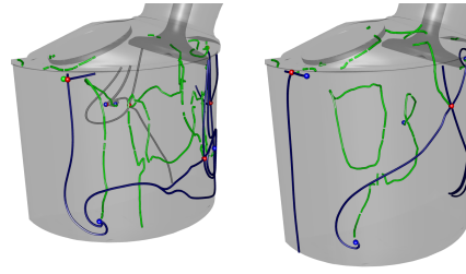
Fig. 8. Two frames from a time-varying visualization of tumble motion using a combination of cutting-plane topology (green lines) and boundary topology (blue lines). Where the critical point paths computed over the cutting-plane parameter range intersect the boundary, singularities appear there, too. This is a prime example of a hybrid approach being used to investigate the relationship between boundary and volume methods.
