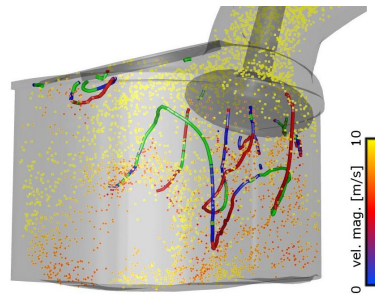
Fig. 2. A frame from a time-varying tumble motion visualization using a combination of particles and vortex cores (lines, extracted by cutting-plane topology). Particle velocity magnitude is color-coded. Lines are colored according to path type (saddles - red, sources - green, sinks - blue). In this frame, some of the particles have been captured in the vicinity of vortex cores resulting in lost energy (lower velocity) for the creation of the tumble pattern.
