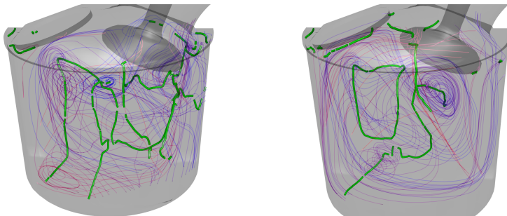
Fig. 5. Two frames from an animation of the tumble motion simulation. Cutting plane topology is applied to visualize flow field structures in the plane orthogonal to the tumble axis. Color of separatrices varies from blue to red on successive cutting planes. Tumble-like flow structures emerge clearly from the otherwise incoherent lines. The paths of critical points over the cutting plane continuum are displayed in green. In the last frame (right), the diagonal main tumble axis can be observed together with a large recirculation zone (closed path on the left).
