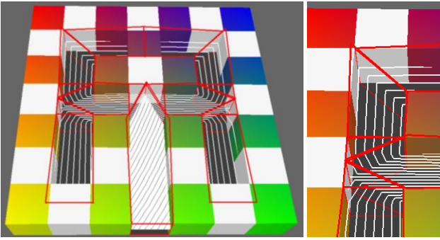
Figure 9. Graph camera model visualization. The frusta are shown in red and few rays are shown in white.
