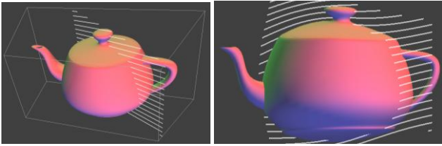
Figure 4. Visualization of rays in 3-D (left) and of their curved projection on the non-pinhole depth image (right) used in Figure 1.
