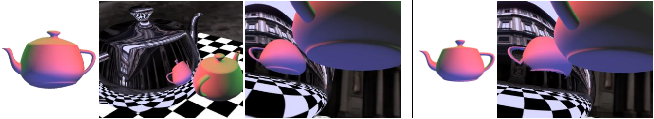
Figure 1. Non-pinhole depth image of teapot and reflections rendered with it (left), and conventional depth image and reflection rendered with it (right). The non-pinhole depth image captures the lid and bottom of the teapot and produces quality reflections.
