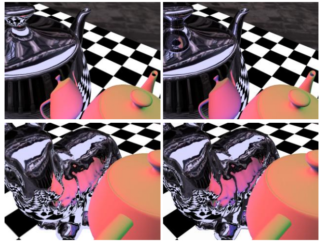
Figure 15. Comparison of our method (left) to ray tracing (right).
