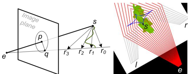
Figure 14. Screen-space ambient occlusion algorithm (left) and visualization of graph camera model (right) used in Figure 3.
