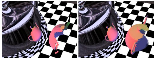
Figure 8. Visualization of samples stored by conventional (left) and SPOC (right) depth image.
