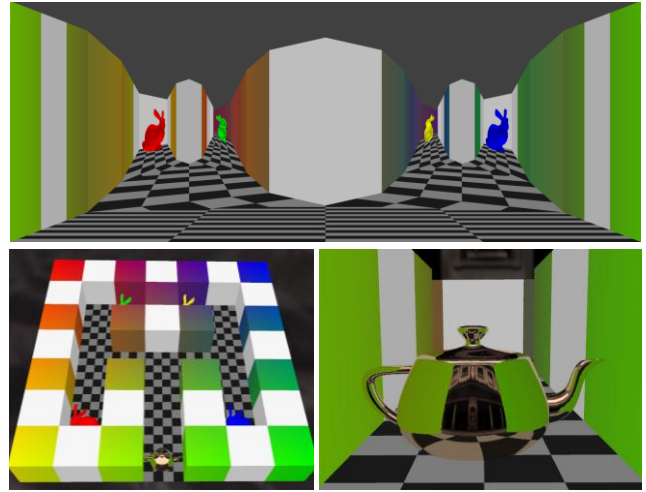
Figure 6. Graph camera depth image (top) capturing an entire 3-D maze (bottom left) and reflection rendered using it (bottom right).
