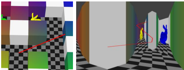
Figure 10. Visualization of 3-D ray (left) and its piecewise linear projection in a graph camera image (right).
