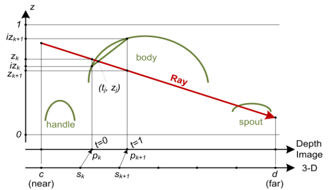
Figure 7. Ray / non-pinhole depth image intersection.
