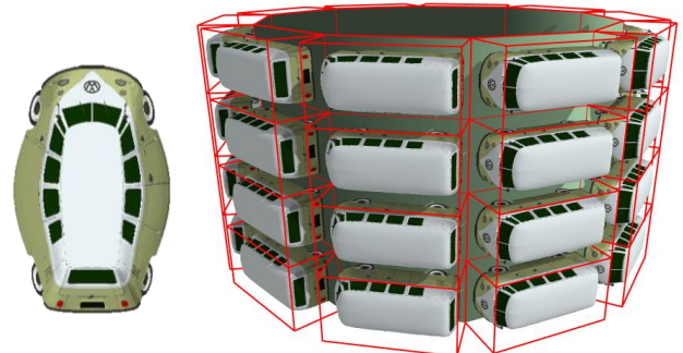
Figure 12. SPOC relief texture (left) and output image with relief bounding box visualization (right).
