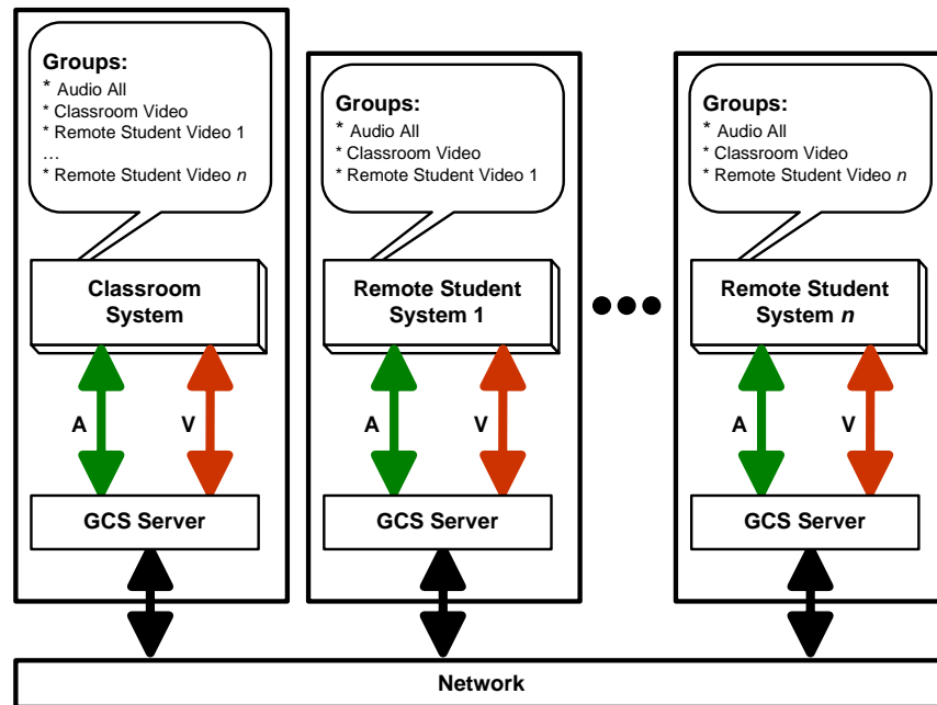
Figure 3. System architecture.
