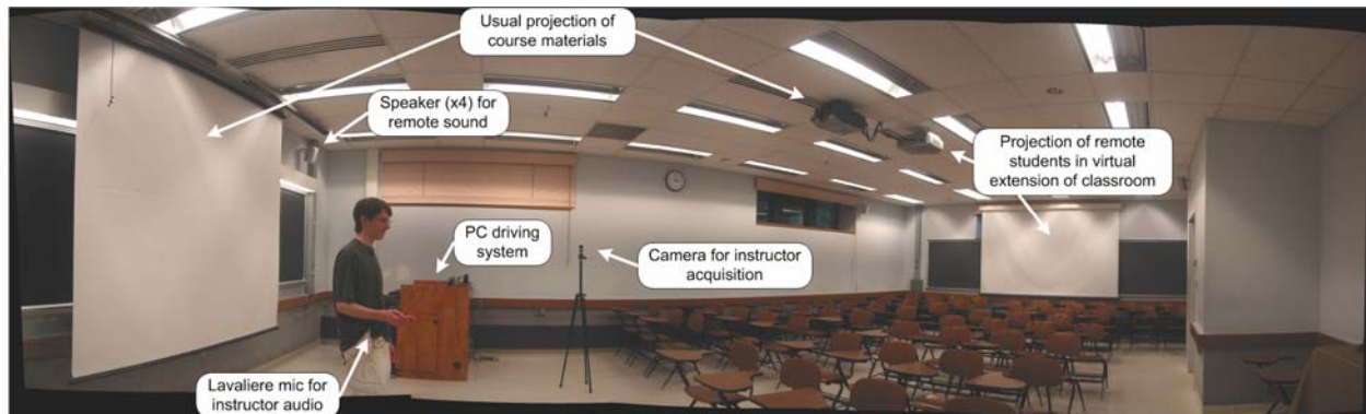
Figure 2. Hardware components for classroom system.
