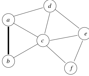
Figure 1. Constraint graph with vertices of weight 2 and edges of weight 1. The minimal dense subgraph \{a, b\} can be extended sequentially by the other elements, in alphabetic order.
