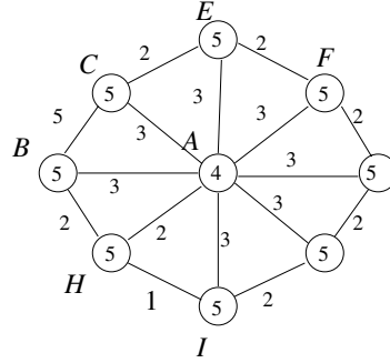
Figure 8. 1/n worst-choice approximation factor of MFA.
