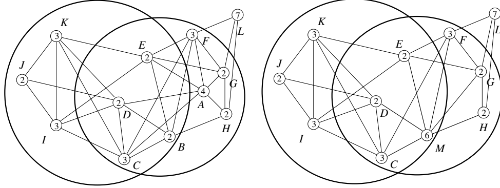
Figure 7. Original graph BCDEIJK is dense, new graph MCDEIJK is not.
