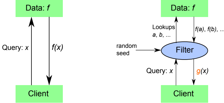
FIG. 1.1. Property-preserving filter. Given a query x , based on a few lookups into the data function f , the filter outputs g(x) , where the function g satisfies a desired property. Notice that if the client makes the same query twice, the filter must return the same value.
