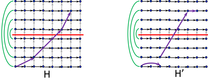
FIG. 4.5. An illustration to the proof of Lemma 4.6: an example transformation from H to H' . Green arches connected matched lines.
