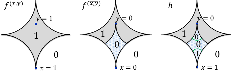
FIG. 3.1. Functions defined in the proof of Theorem 1.4: f^{(x,y)}(v) , f^{(\bar{x},\bar{y})} and H .
