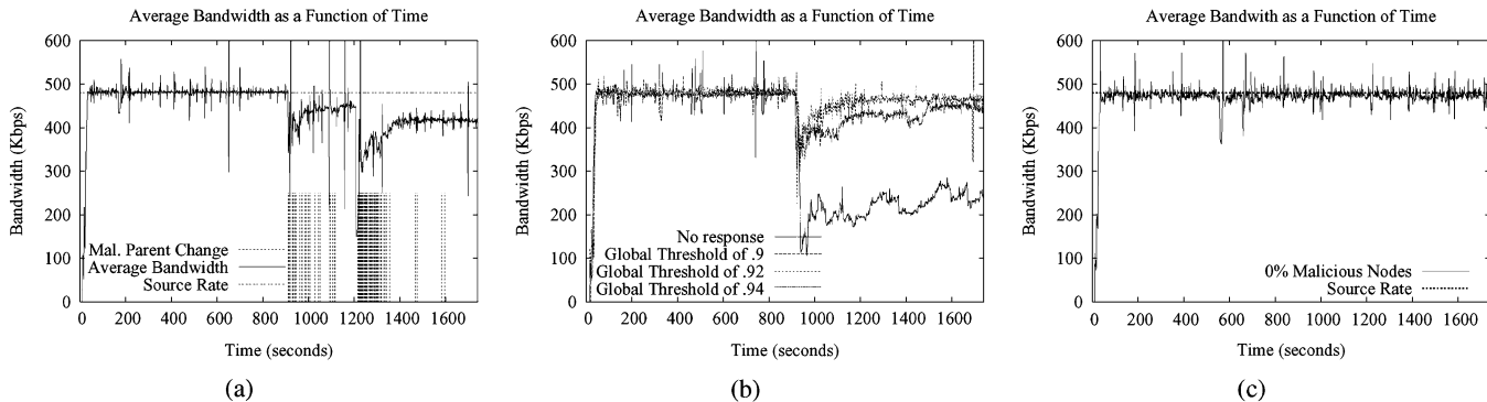
Fig. 7. (a) Effectiveness of local response in mitigating attacks on an ESM overlay of 100 nodes on PlanetLab for a duration of 30 min. (b) Effectiveness of global response in mitigating attacks on an ESM overlay of 100 nodes on PlanetLab for a duration of 30 min. (c) Average bandwidth over time for an ESM overlay of 100 nodes on PlanetLab for a duration of 30 using both response mechanisms under non-attack conditions.
