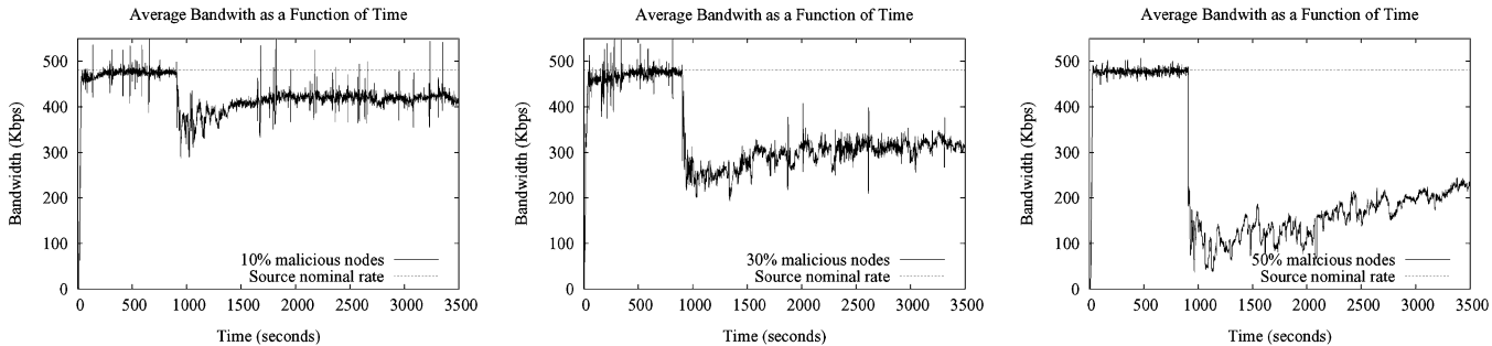
Fig. 4. Average bandwidth over time for an ESM overlay of 100 nodes on PlanetLab for a duration of 60 min with different percentages of malicious nodes.
