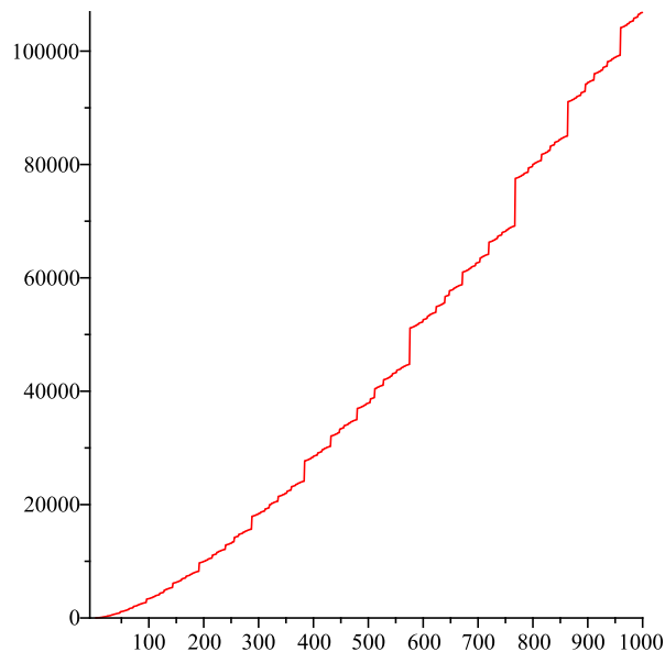
Figure 1: T(n) versus n from Example 1.
