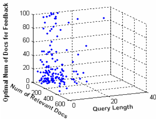
Figure 2. Query feedback behavior distribution for the CMU system, showing the relationship between number of relevant documents or query length with the optimal number of documents for feedback. (Mainly from the point of view of the number of relevant documents.)
