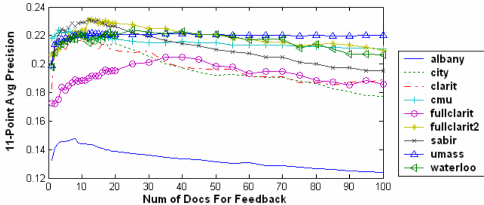
Figure 1. Performance across systems when varying the number of documents used for feedback
