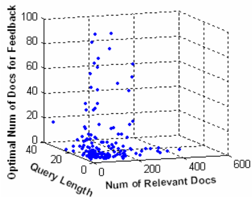
Figure 3. Query feedback behavior distribution for the Fullclarit2 system, showing the relationship between query length or number of relevant documents with the optimal number of documents for feedback. (Mainly from the point of view of query length.)
