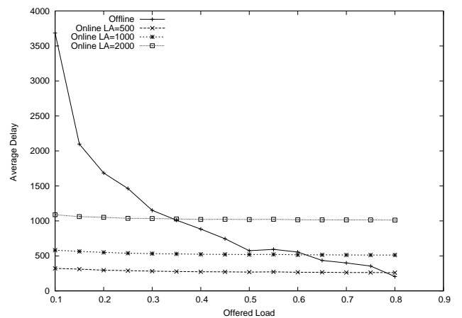
Figure 8: Average packet delay for both online and offline algorithms under bursty arrivals.
