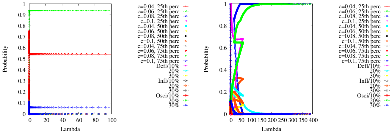
(a) Game 3 (b) Game 4 Fig. 4. The Quantal Response Equilibrium evaluation for the King data set
