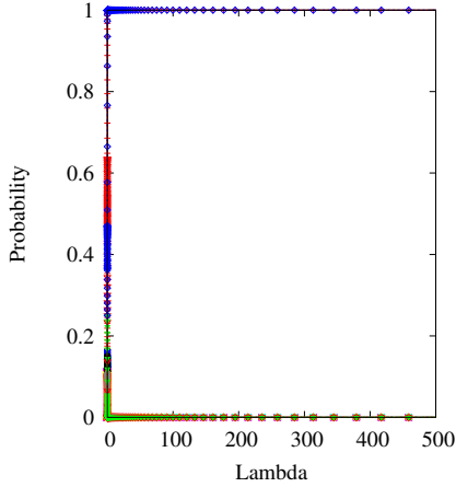
(a) Prediction error
