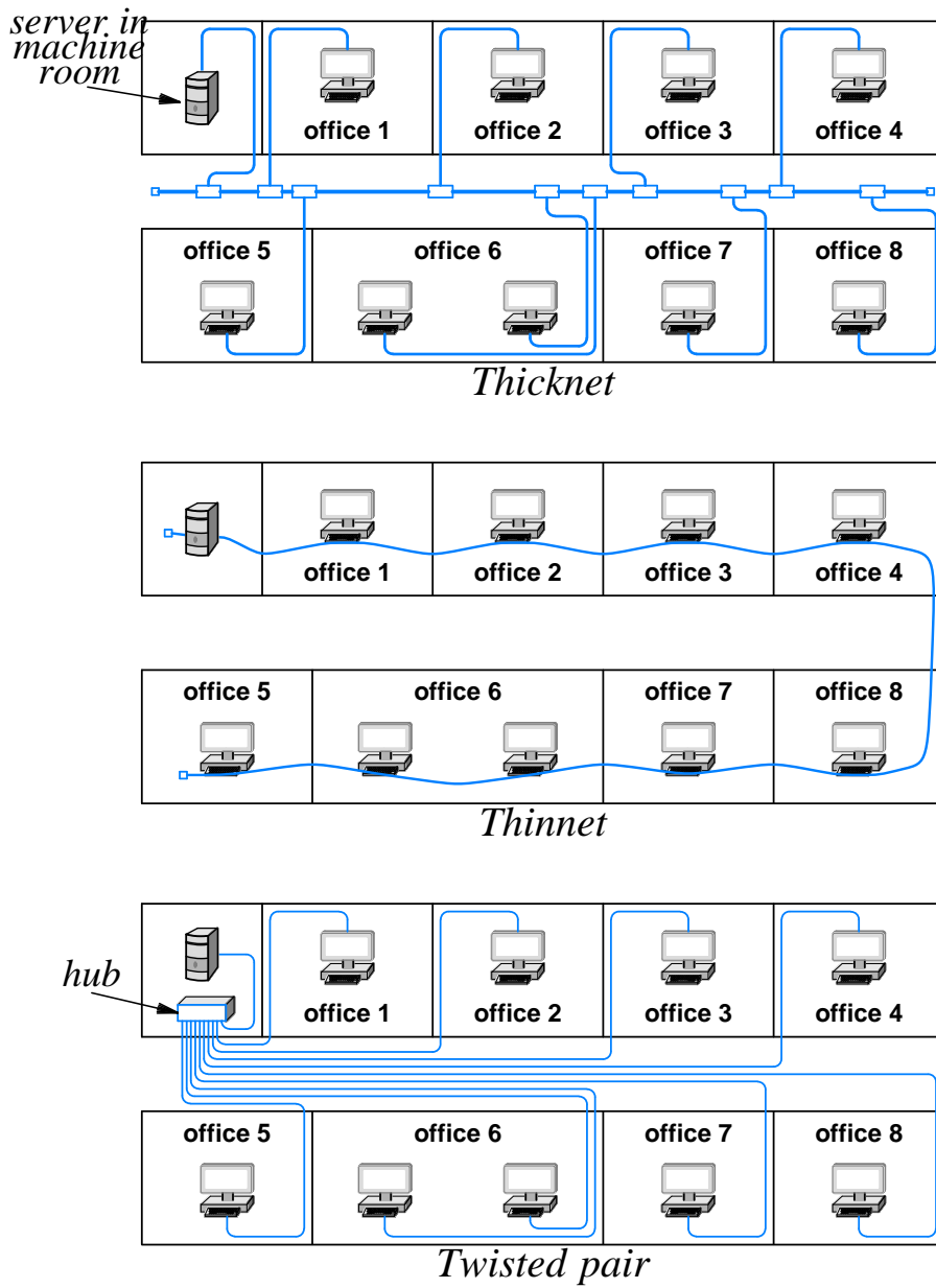
Figure 15.7 Illustration of various LAN wiring schemes that have been used in an office building.
