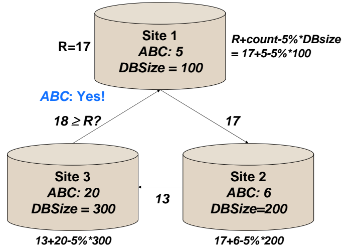
Fig. 2. Determining if itemset support exceeds 5% threshold
