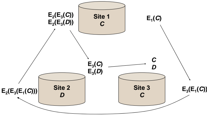
Fig. 1. Determining global candidate itemsets
