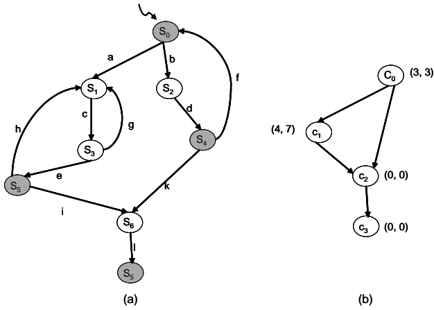
Figure 2: A transition system (a) with its \mathcal{G}^{scc} (b)
