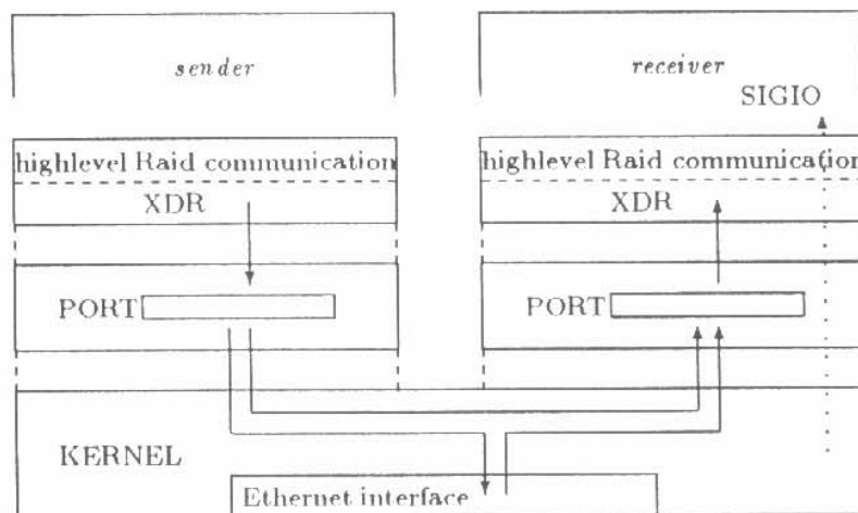
Figure 4. The structure of Raidcomm V.2
