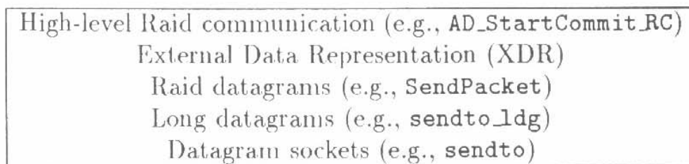
Figure 1. Layers of the Raid communication package version 1.
