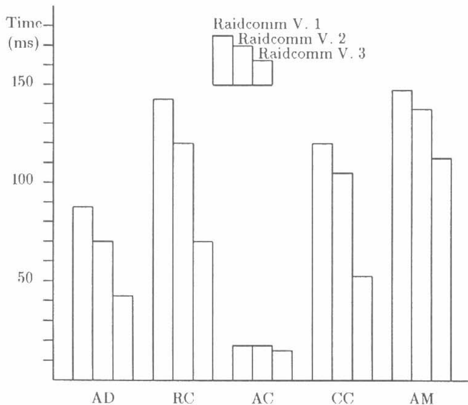
Figure 13. User times for Raid servers (ms)
