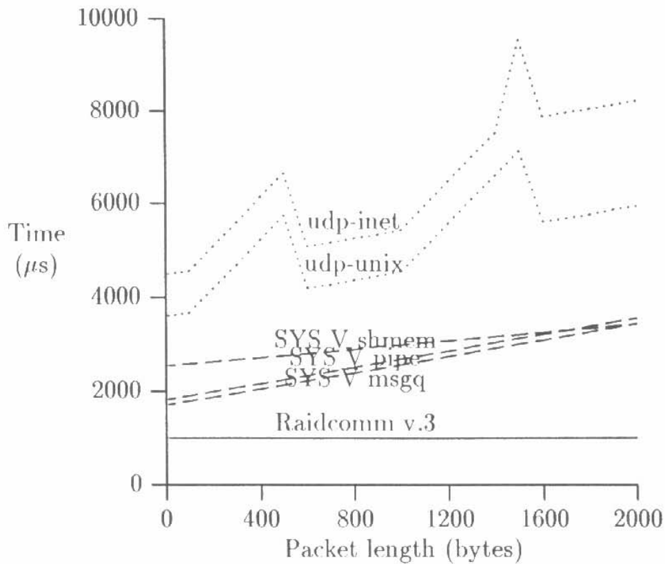
Figure 12. Comparison of message round trip times
