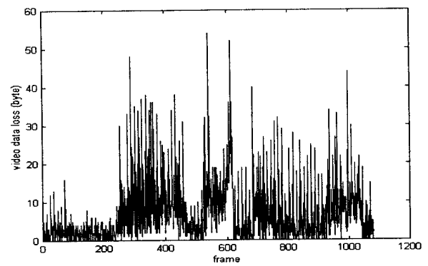
Fig. 3. Video data loss without error control (BER=0.01, Average data loss = 6.5 bytes/frame)
