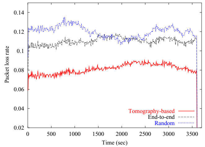
Fig. 8 Aggregated loss rate perceived by the receiver: with peer failures
