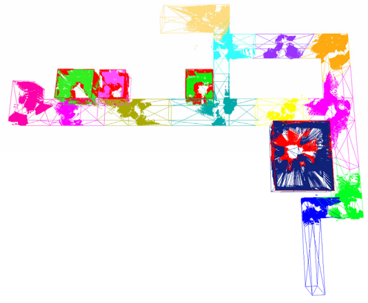
Figure 8: This floor consists of 12 corridor and 4 rooms sections. The point clouds used to build the corridor sections are also shown.
