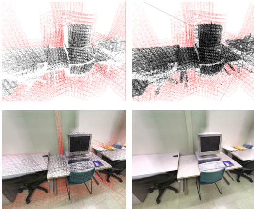
Figure 5: Points lying within threshold distance to the fitted box are marked as invalid (red). Triangles connecting all invalid points are discarded, leaving only triangulation of the fragmented geometry. A complete room model is a union of fragmented geometry and fitted section triangles (bottom right).
