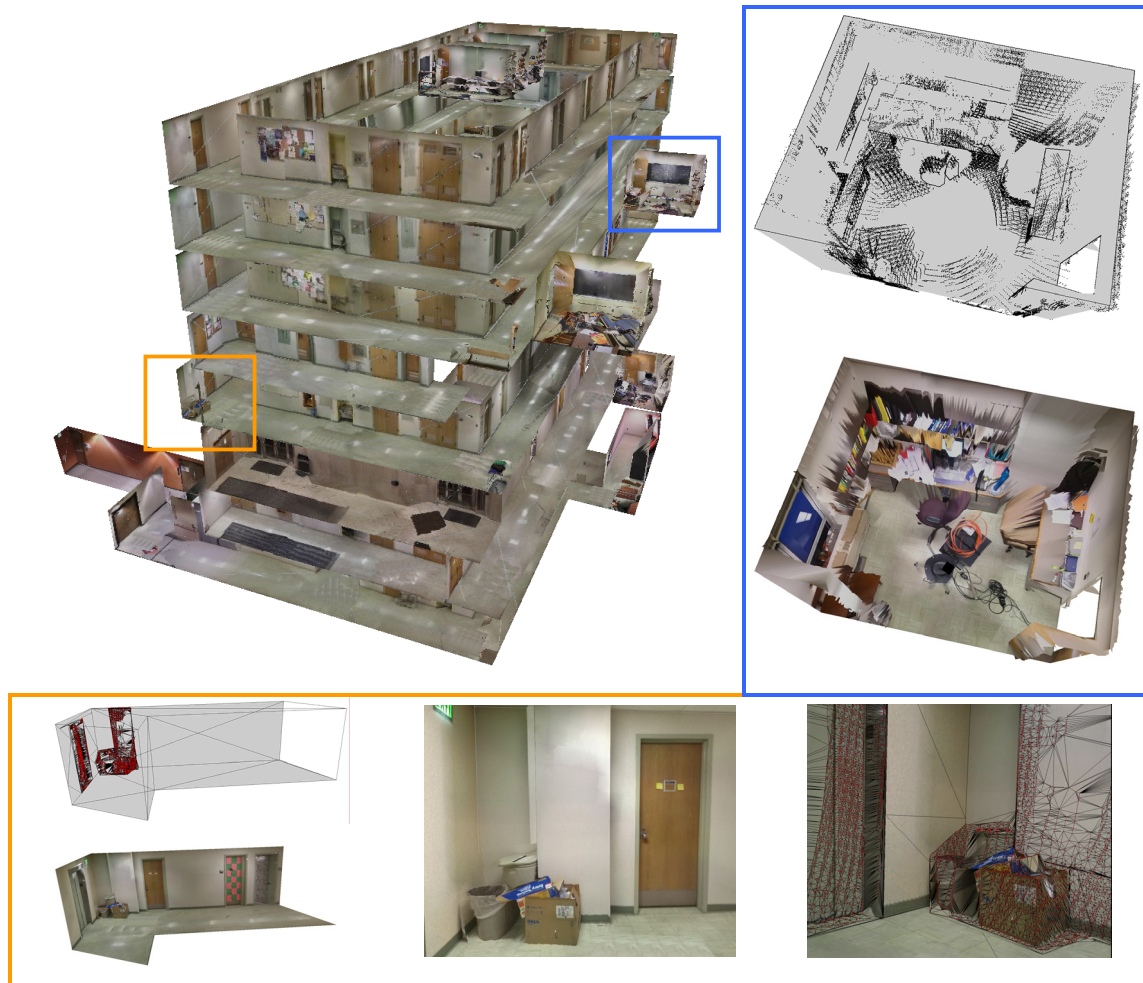
Figure 1: This model was acquired in 40 hours by a two person team using a single acquisition device. The model spans 6 floors with 20 attached rooms. Individual rooms (see blue) and corridors (see orange) are modeled with fitted proxy geometry enhanced with embedded detail.
